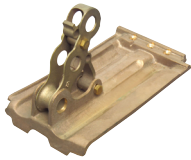
MULLANE FITRITE #631 & #632 SNOW FENCE BRACKET - FRENCH TILE
