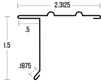
F5M DRIP EDGE CONTINUED
