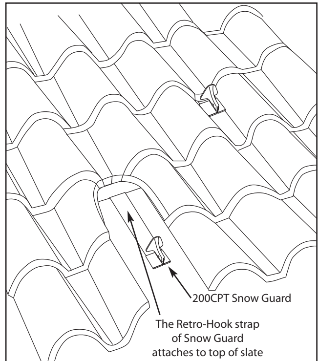
Typical Snow Guard spacing on Spanish tile roofing.
