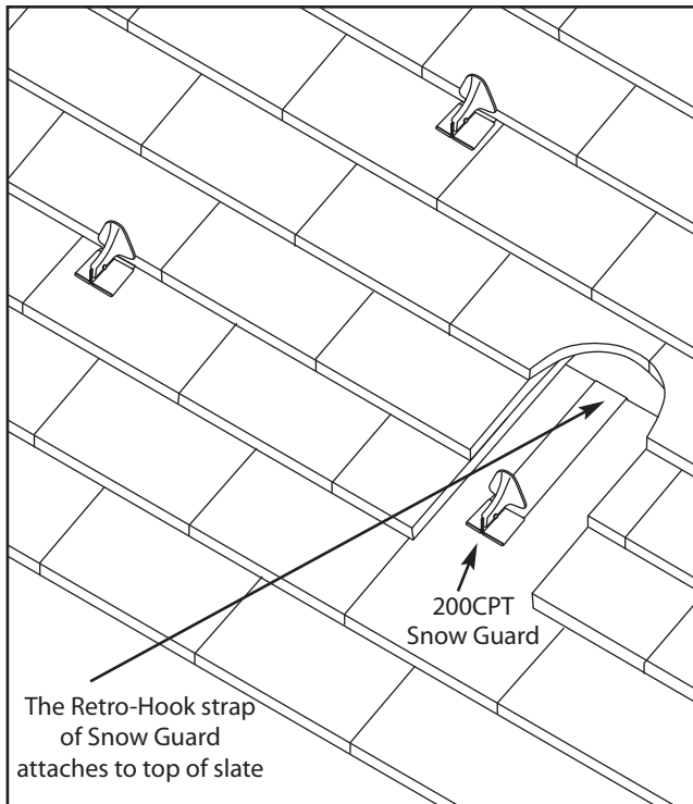
Typical Snow Guard spacing on flat tile roofing.
