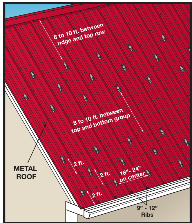
Adhesive Layout
