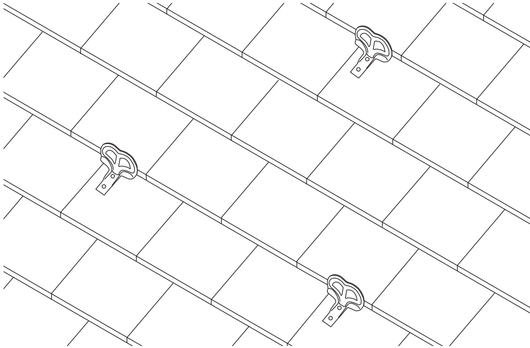
Correctly spaced Snow Guard on 1/2" thick slate. Cap is 1-1/2" from front edge of slate in course.
